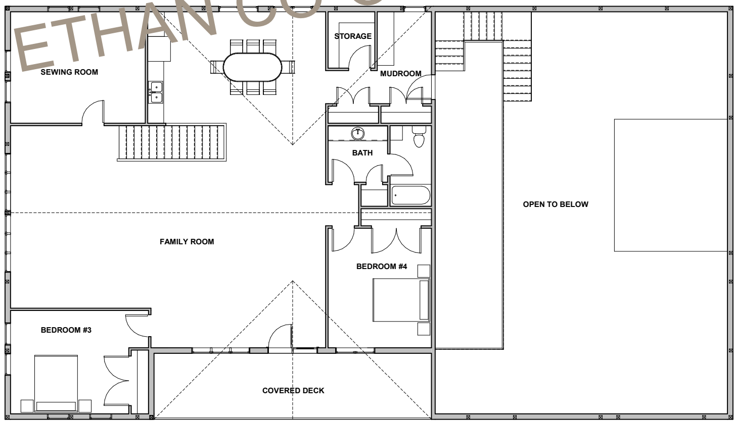
② Second Floor 3/16" = 1'-0"
