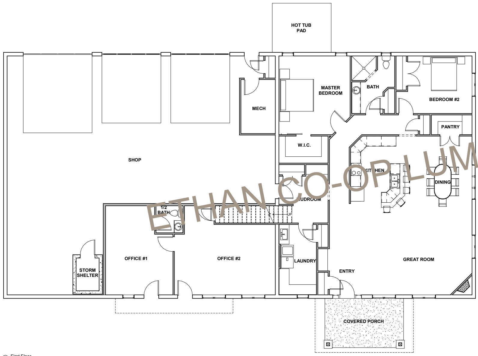
① First Floor 3/16" = 1'-0"
