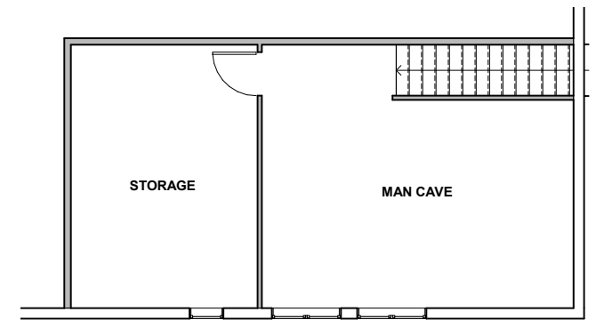
② Second Floor 3/16" = 1'-0"
