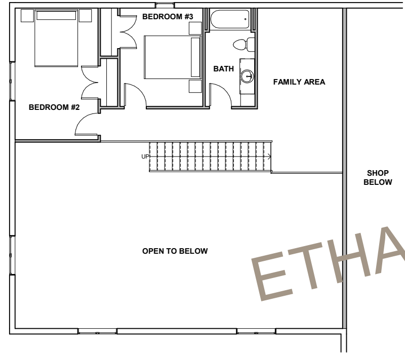
② Second Floor 3/16" = 1'-0"
