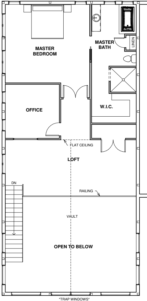
① Second Floor 3/16" = 1'-0"
