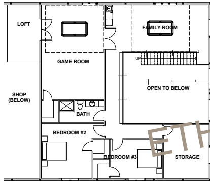
② Second Floor 1/8" = 1'-0"
