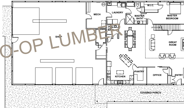
① First Floor 1/8" = 1'-0"
