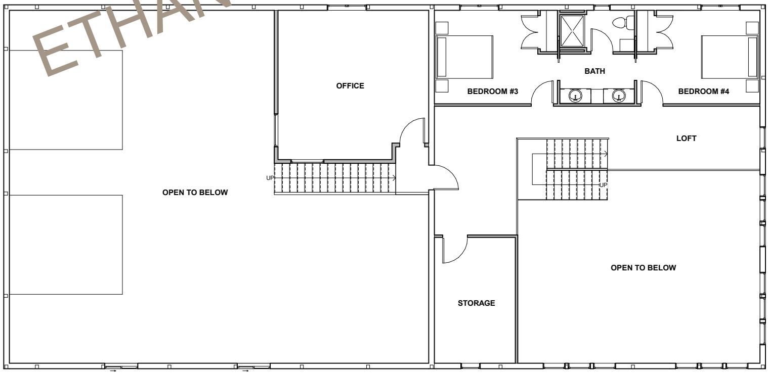
② Second Floor 3/16" = 1'-0"
