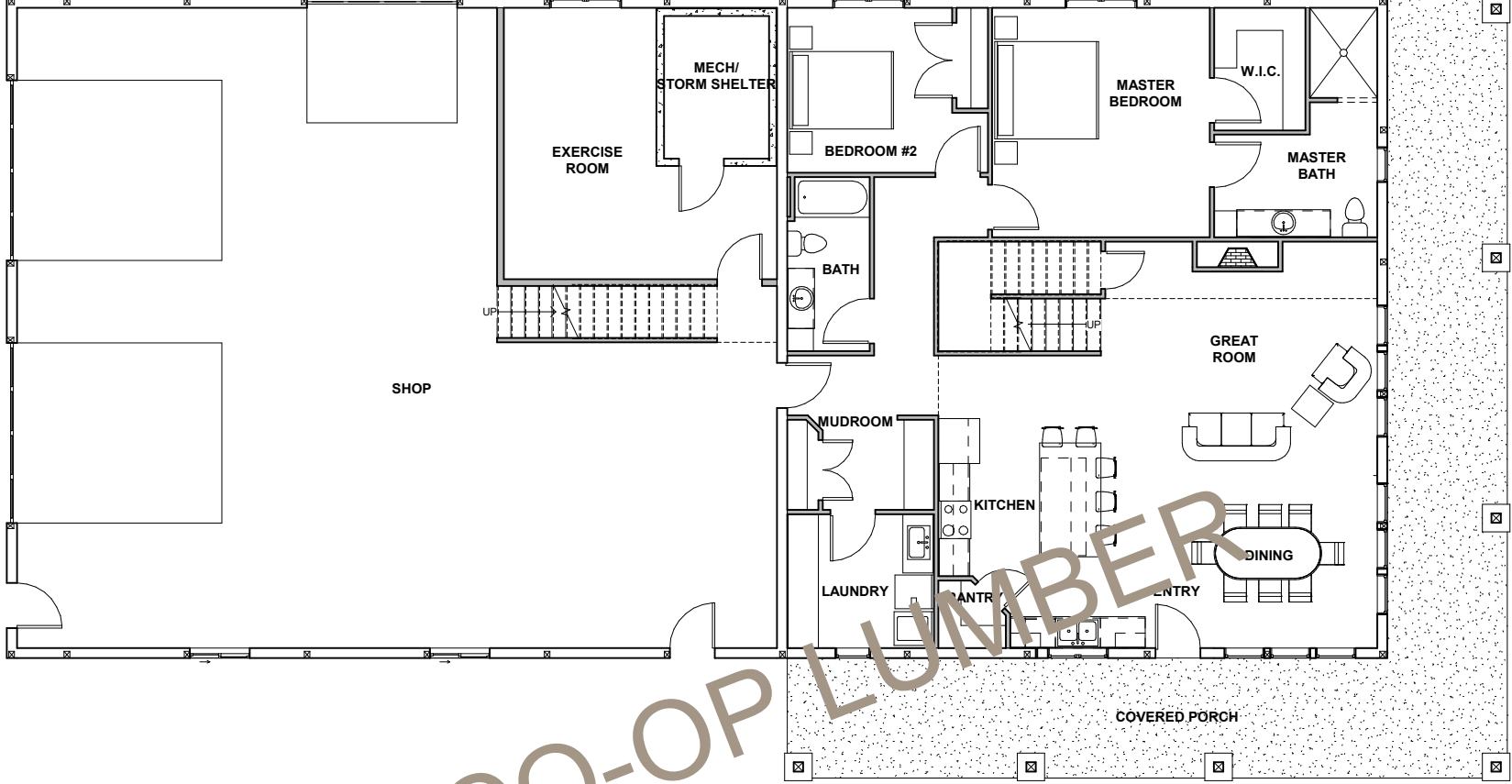
① First Floor 3/16" = 1'-0"
